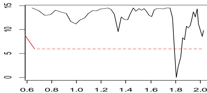
Figure 1. Confidence interval construction of threshold
